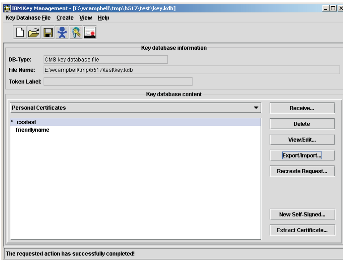
Figure 8. Personal Certificates in CMS key database after import
